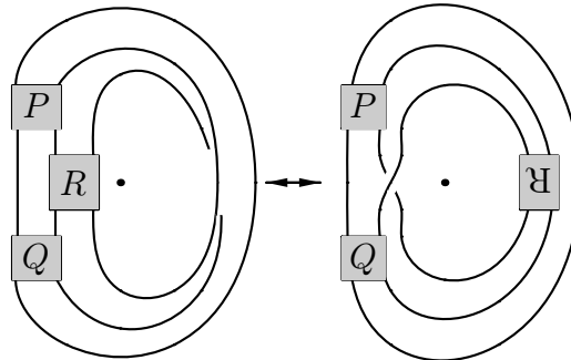
Figure 1.84.3. Simplest generalized flype
